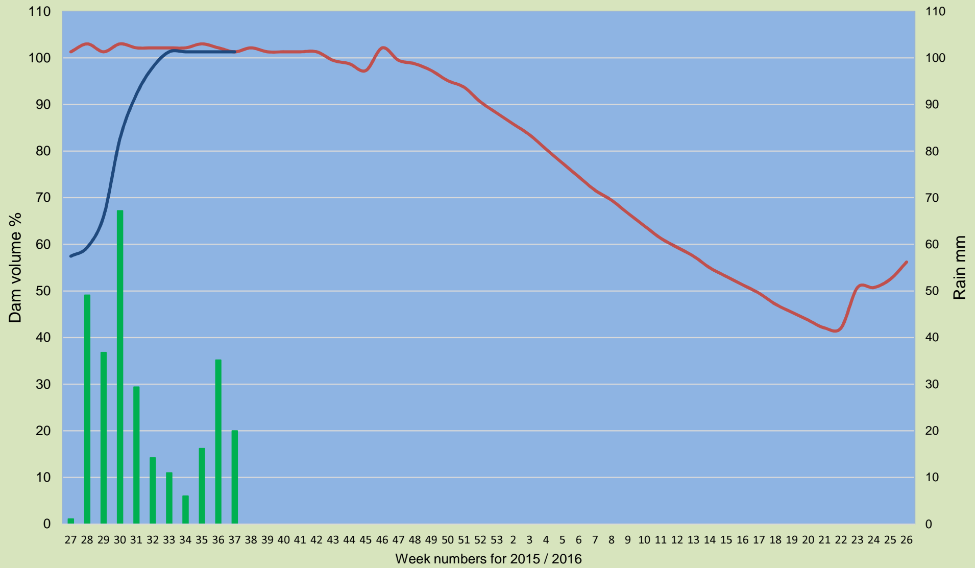
Eikenhof dam volume % and rain millimetre
